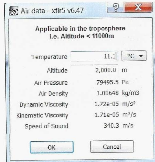
Gambar 9. Aero Data Variable
